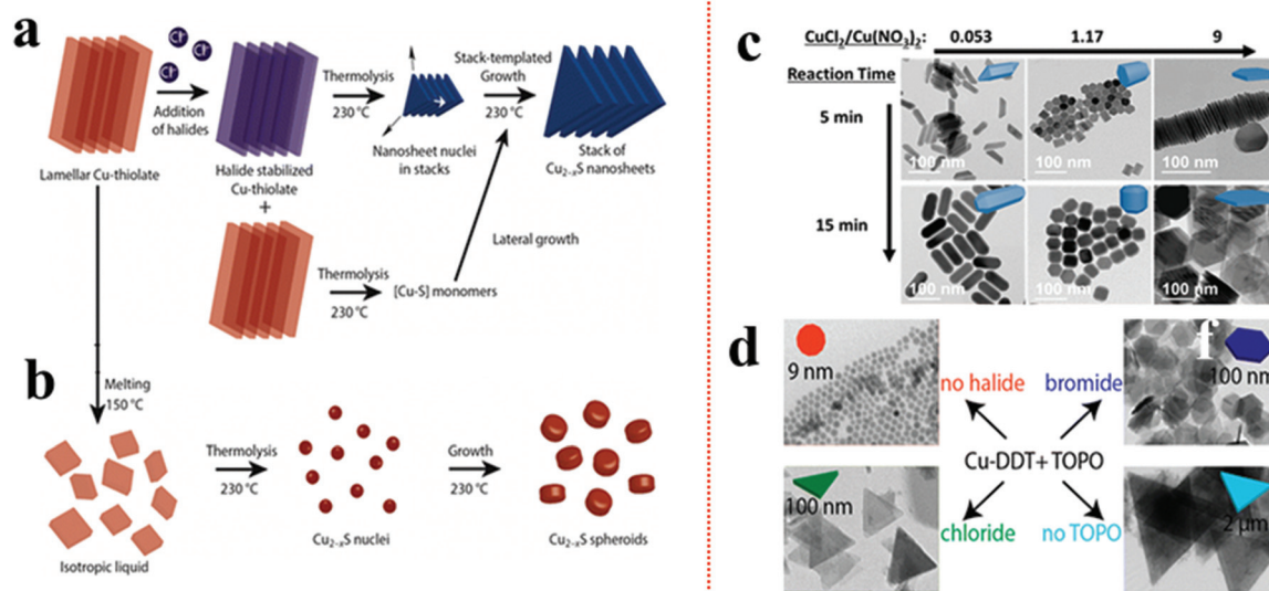
Fig. 1 (a) Schematic of controlling the 2D shape of the \text{Cu}_{2-x}\text{S} using \text{Cl}^- source. The \text{Cl}^- stabilized the lamellar Cu-alkanethiolate structure close to the nucleation stage influencing a 2D templated nucleation; (b) in the absence \text{Cl}^- the lamellar structure melts and provides monomers for \text{Cu}_{2-x}\text{S} nuclei formation resulting in spheroids. Reproduced from ref. 49 with permission from ACS, copyright 2016; (c) effect of ratio variation between \text{CuCl}_2 and \text{Cu}(\text{NO}_3)_2 on morphology control of \text{Cu}_{2-x}\text{S} . Reproduced from ref. 90 with permission from ACS, copyright 2017; (d) effect of \text{SnX}_4 ( X = \text{Cl}, \text{Br} ) additives on nanoplate formation of \text{Cu}_{2-x}\text{S} . The \text{Br}^- source formed hexagonal plates whereas the \text{Cl}^- source produced triangular plates. Reproduced from ref. 91 with permission from ACS, copyright 2016.
