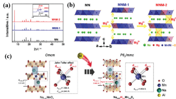
Fig. 4 (a) XRD and (b) structural evolution of Mg doped \text{Na}_{0.7}[\text{Mn}_{0.6}\text{Ni}_{0.4-x}\text{Mg}_x]\text{O}_2 (MNM- x ); adapted with permission. 40 Copyright 2018, American Chemical Society. (c) Schematic illustration of effects of \text{Al}^{3+} doping on electrode structures. Adapted with permission. 48 Copyright 2019, Wiley-VCH.
