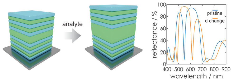
Fig. 7 Left: Schematic illustration of a defect layer embedded in a 1DPC. Right: Calculated resulting drop in the reflectance caused by the defect in a 1DPC. The RI of the low RI material was n_l = 1.5 and n_h = 2.0 for the high RI material and the defect was embedded in the middle ( n = 1.5 , d = 160 nm) of the 6 bilayers comprising the 1DPC. After analyte exposure the thickness of the defect layer was 240 nm. Note that the reflectance was calculated for a glass substrate with n = 1.51 and a thickness of 1mm. The thickness of each layer in the 1DPC was 80 nm.
