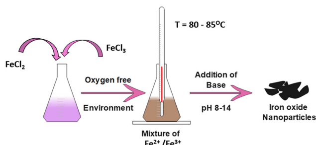
Fig. 3 Steps to synthesize IONPs through the co-precipitation method. \text{Fe}^{2+} and \text{Fe}^{3+} are added in a 2:1 molar ratio in an oxygen-free environment and heated to 80–85 °C followed by the addition of base. The precipitated particles are then centrifuged or magnetically separated.
