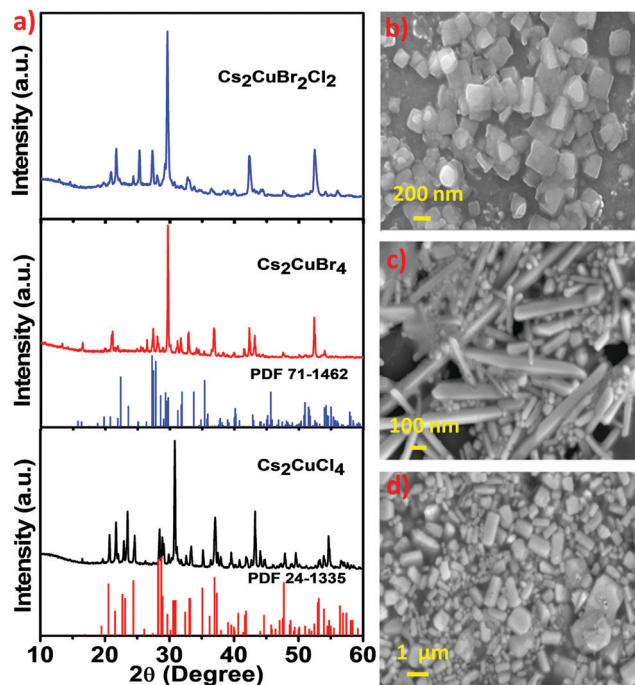
Fig. 3 (a) X-ray diffraction pattern of \text{Cs}_2\text{CuCl}_4 , \text{Cs}_2\text{CuBr}_4 and \text{Cs}_2\text{CuBr}_2\text{Cl}_2 . (b–d) SEM images of \text{Cs}_2\text{CuCl}_4 , \text{Cs}_2\text{CuBr}_4 and \text{Cs}_2\text{CuBr}_2\text{Cl}_2 present square shaped nanoplates, nanorods and rectangular shaped nanoplates, respectively.
