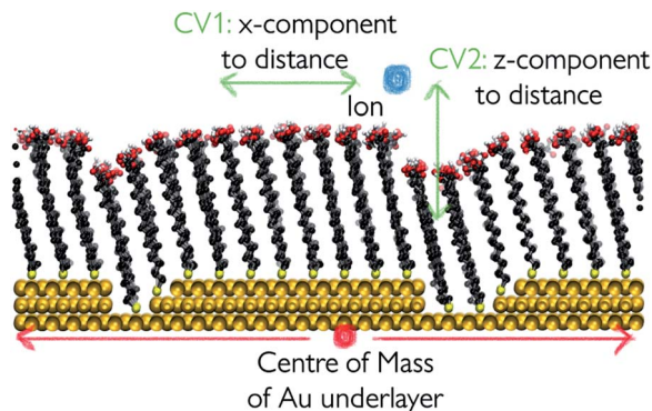
Fig. 3 Schematic representation of the collective variables used to apply WTmetaD. The distance between the centre of the outermost Au layer and the centre of the ion is broken down into x - y - and z -components. Bias is applied on the x - and z -components.
