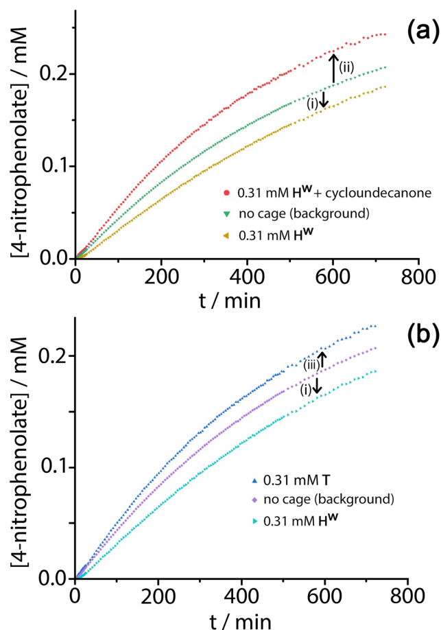
Fig. 8 Contributions of \text{H}^{\text{W}} and T to positive and negative catalysis of 4NPA hydrolysis (0.3 mM 4NPA, pH 7.4, 303 K). Panel (a) shows the retardation effect (negative catalysis) of \text{H}^{\text{W}} on 4NPA hydrolysis [arrow (i)] associated with cavity binding, and the small acceleration [arrow (ii)] associated with external surface based catalysis when the cavity is blocked using cycloundecanone. Panel (b) shows the contrasting effects of \text{H}^{\text{W}} [arrow (i), as before] and T [arrow (iii)] in which no cavity binding of the 4NPA is possible and only external-surface catalysis can occur.
