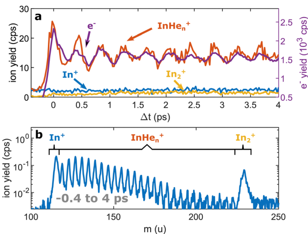
Fig. 2 Pump-probe photoionization of In 2 inside He N at short time delays showing the initial WP oscillation. (a) Transient photo-ion signals for different mass channels, in comparison to the transient photoelectron signal. 15 (b) Ion mass spectra obtained through integration of the transient signals up to 4 ps.
