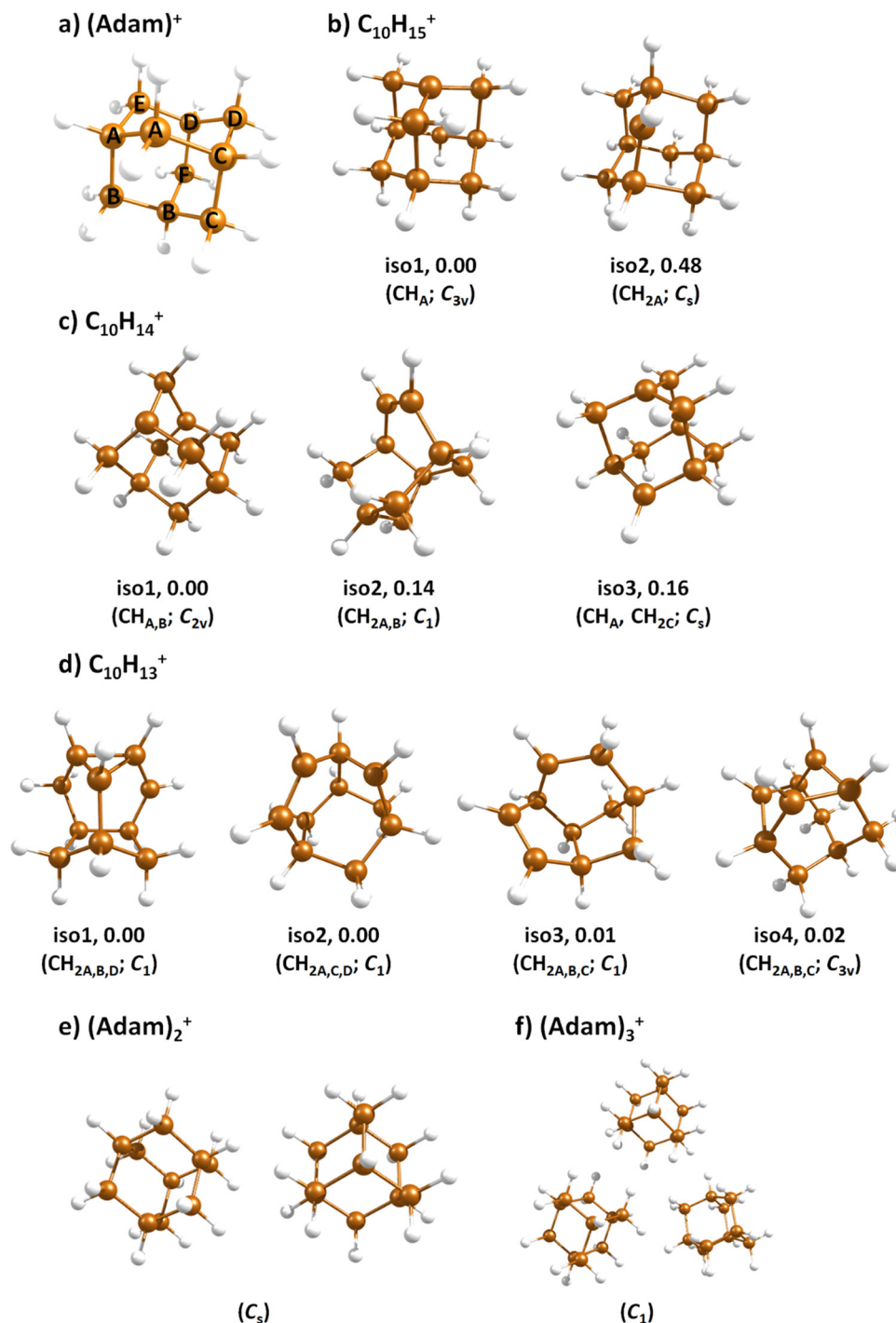
Fig. 3 Selected isomers of (a) Adam + , (b) C 10 H 15 + , (c) C 10 H 14 + , (d) C 10 H 13 + , (e) (Adam) 2 + , and (f) (Adam) 3 + optimised at the B3LYP+D3/aug-cc-pVDZ level of theory along with the relative isomer energy in eV and symmetry point group. In (b–d), hydrogen atoms removed from CH and CH 2 groups of (Adam) + are denoted according to atom nomenclature shown in (a).
