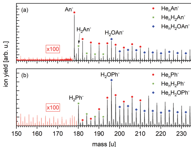
Fig. 3 Sections of negative ion mass spectra of HNDs doped with (a) An and (b) Ph measured in the Clustrof setup. To increase the visibility of the mass range < 180 u, the peaks are multiplied by a factor 100. Labeled mass peaks refer to ions that are isotopically pure (containing ^1\text{H} , ^{12}\text{C} , ^{16}\text{O} ). While the formation of bare \text{An}^- is clearly visible in panel (a), the presence of bare Ph ^- in panel (b) is questionable. For the mass range \geq 180 u, anionic complexes of An or Ph with He, or with \text{H}_2 or \text{H}_2\text{O} plus He atoms are observed. The detected mass peaks in the mass range < 180 u can be linked to He series attached to water clusters.
