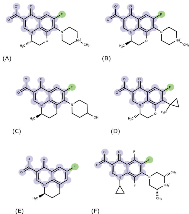
Fig. 1 Examples of FQ structures: (A) levofloxacin (LFX), (B) ofloxacin (OFX), (C) nadifloxacin (NFX), (D) pazufloxacin (PFX), (E) flumequine (FMQ), and (F) orbifloxacin. The molecular scaffold common to all quinolones and the fluorine atom characterizing fluoroquinolones are highlighted in blue and green, respectively.
