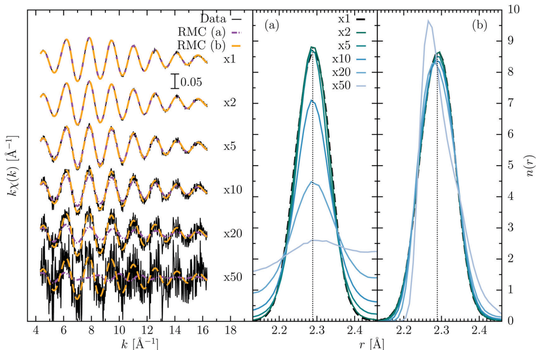
Fig. 2 RMC refinement of \text{Br}_2 data adding increasing levels of noise. On the left, the synthetic data and the RMC simulations are shown, where the labels indicate the multiplier respect to the original noise in the data ( \sigma^2 \sim 10^{-6} ). Two different approaches have been used: for case (a), the noise used in the RMC procedure reflected the correct estimation of the noise in the data, while for case (b) the original value of noise ( \sigma^2 \sim 10^{-6} ) was used. The number distribution functions n(r) obtained for the different data and the two approaches are shown on the right. For case (a), the distribution remains centered around the same value, becoming very broad as the noise increases. For case (b), instead, there is no visible broadening effect, but the peak becomes slightly distorted and skewed.
