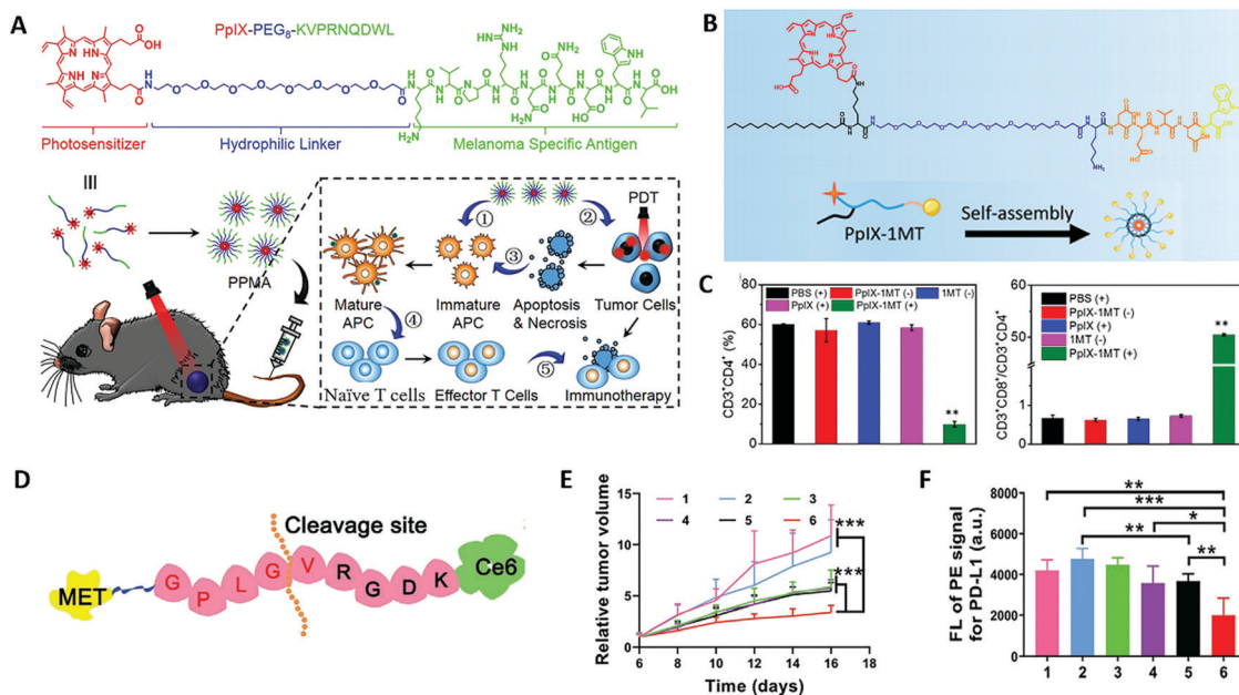
Fig. 2 (A) The chemical structure and the proposed mechanism of PpIX-PEG 3 -KVPNRQDWL for photodynamic therapy amplified immunotherapy against melanomas. Adapted with permission from ref. 57. Copyright 2021 John Wiley and Sons. (B) Structure of the chimeric peptide PpIX-1MT. (C) Ratio of CD4 + T cells to CD3 + lymphocytes and ratio of CD3 + CD8 + T cells to CD3 + CD4 + T cells after different treatments. Adapted with permission from ref. 41. Copyright 2021 American Chemical Society. (D) The design of self-delivery NPs for combination breast cancer immunotherapy. (E) Change in relative tumor volume during the treatment. (F) Expression of PD-L1 in tumor cells after various treatments were determined by flow cytometry. Adapted with permission from ref. 62. Copyright 2021 John Wiley and Sons.
