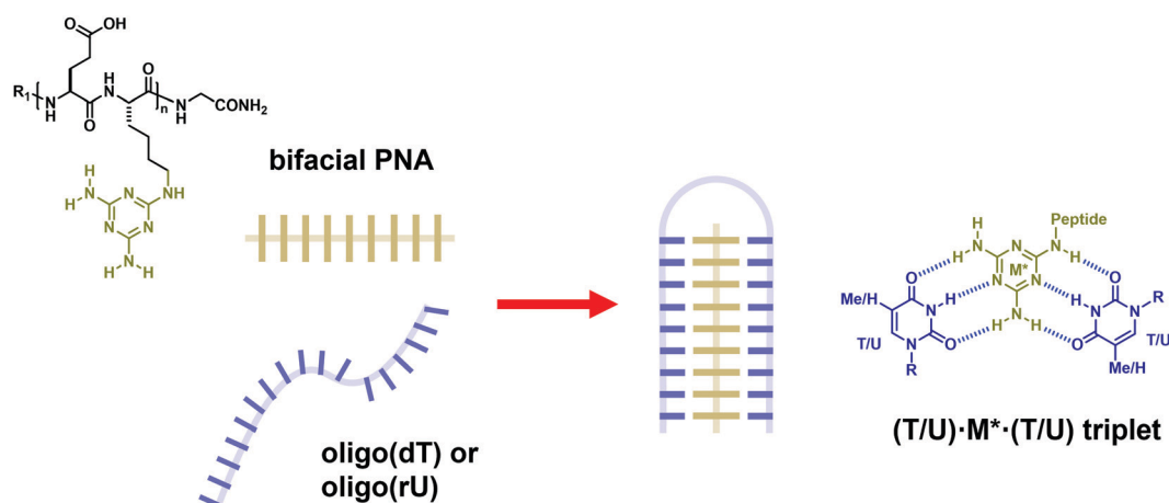
Fig. 39 Structures of bifacial PNA containing the melamine base (gold) and its interaction with thymine in DNA (blue) or uracil in RNA strands to form a stable triplet structure (adapted with permission from ref. 200. Copyright 2012 American Chemical Society).
