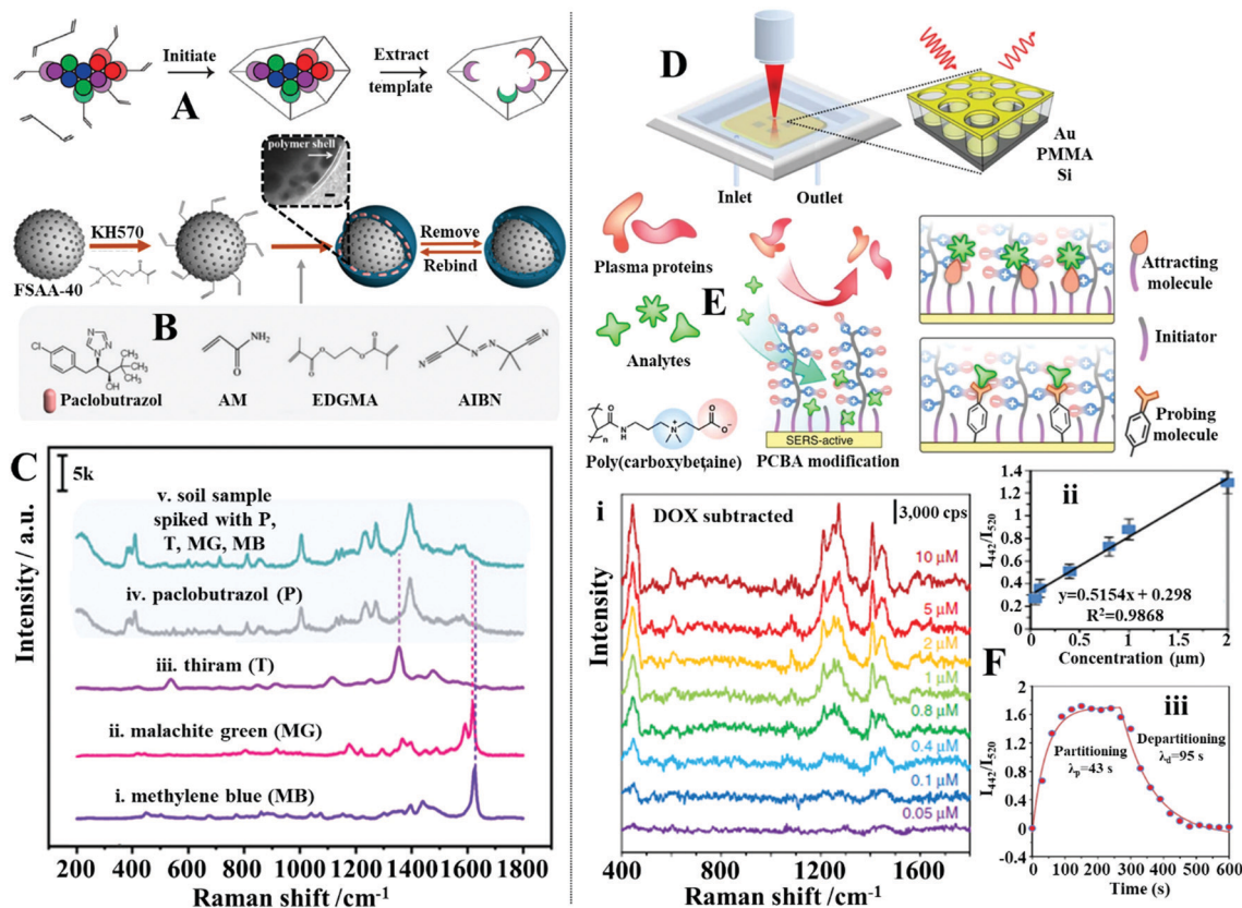
Fig. 12 (A) Schematic illustrations of the working principles of molecular imprinted polymers (MIPs); (B) schematic illustration of the preparation of \text{Fe}_3\text{O}_4@(\text{SiO}_2-\text{Au}@\text{Ag}) (FSAA) MIPs. Inset shows a TEM image of the product FSAA MIPs; (C) SERS spectra set demonstrating the selectivity of the FSAA MIP sensors. Spectra (i–iv) correspond to the SERS signals of the target analyte paclobutrazol and three contaminants, namely, thiram, malachite green and methylene blue. Spectrum v corresponds to the SERS signals obtained from a soil sample spiked with all four chemicals; (D) schematic illustrations of the SERS optofluidic system; (E) schematic illustrations of the different types of mixed self-assembled monolayers functionalized on the surface of the enhancing material to achieve anti-fouling and target recognition; (F) panel (i) show SERS spectra of Doxorubicin in plasma ultrafiltrate control at concentrations ranging from 0.05 to 10 \mu\text{M} . The background signals from plasma have been subtracted. Panel (ii) shows the linear region of the Doxorubicin detection curve generated by plotting the average intensity ratio of the doxorubicin peak at 442 \text{cm}^{-1} and plasma peak at 520 \text{cm}^{-1} as a function of doxorubicin concentration. The error bars stand for standard deviations obtained from three replicates. Panel (iii) shows partitioning and departitioning kinetics of 20 mM Doxorubicin in plasma on the anti-fouling SERS sensor. Panel (A) reproduced with permission from ref. 178, copyright 2017 American Chemical Society. Panel (B and C) adapted with permission from ref. 75, copyright 2020 American Chemical Society. Panel (D–F) adapted with permission from ref. 182, copyright Springer Nature Limited.
