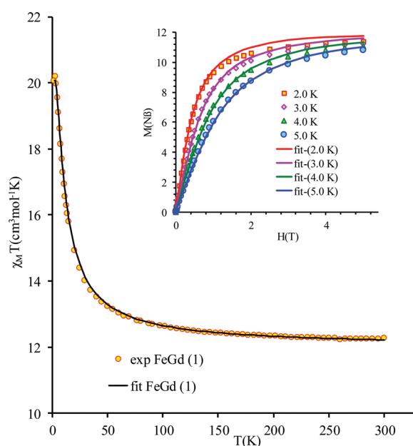
Fig. 3 \chi_{\text{M}}T vs. T curve for compound 1. Inset: Field dependence of the magnetization at various temperatures. The solid lines is the best simultaneous fit of magnetization and susceptibility data based on the anisotropic Hamiltonian (1).
