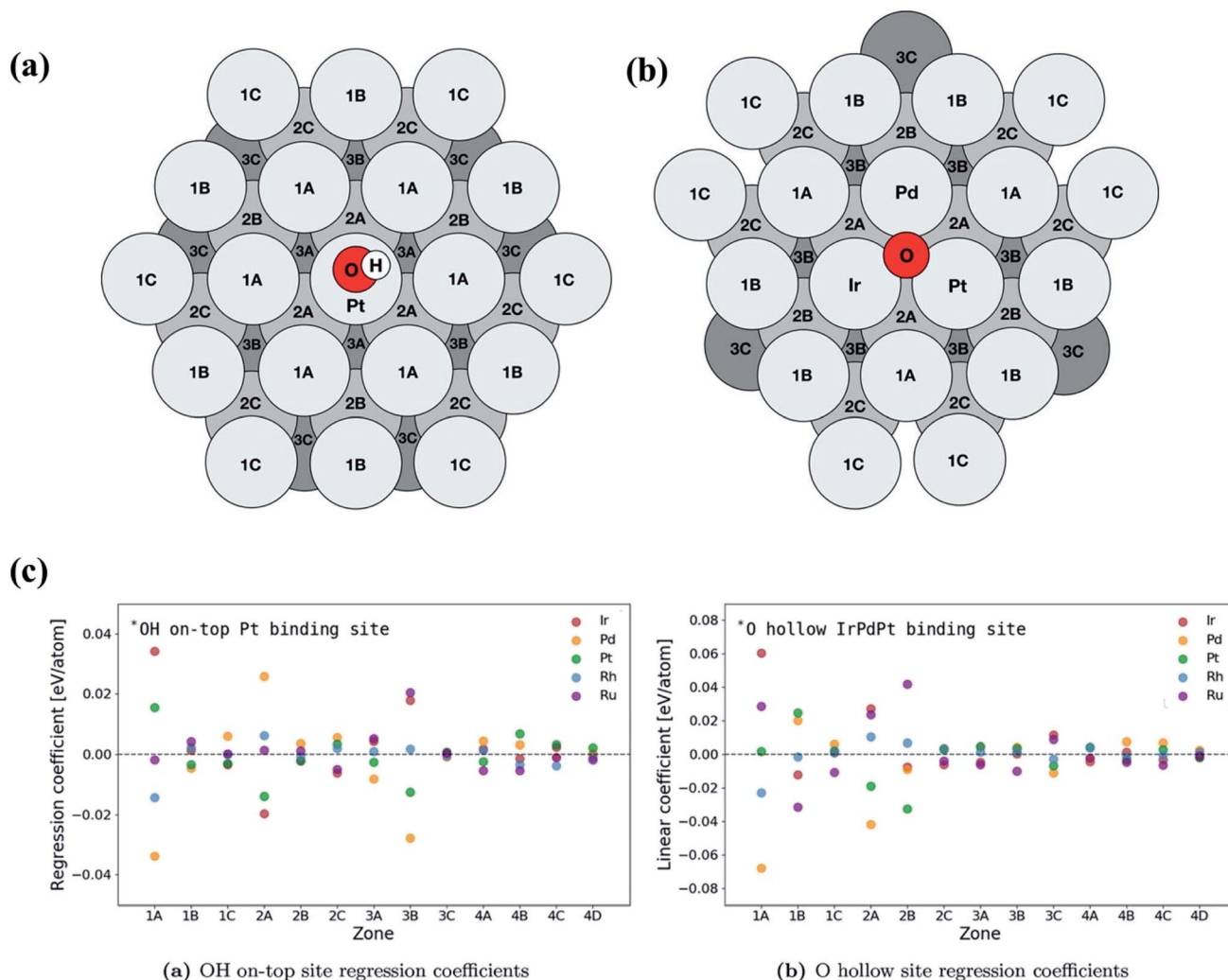
Fig. 16 Schematic of atomic positions grouped by layer and distance from the binding site on an FCC (111) surface microstructure for (a) on-top adsorption on Pt and (b) fcc hollow site adsorption on IrPdPt. The fourth layer contains zones 4A, 4B, 4C and 4D and has an identical layout to the first layer. (c) Overview of the regression coefficients of the least squares fits for each element by zone. The atoms with direct coordination ( i.e. , zones 1A and 2A) to the binding atoms have a large effect on the binding energy of the intermediate. Zone 3B has a similar sized impact on the binding energy to the neighbors in zone 2A. Reproduced from ref. 126 with permission from John Wiley and Sons.
