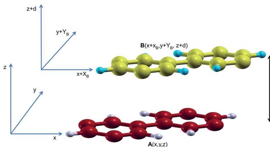
Fig. 1 Bilayer stacking scheme. Cartesian coordinates of the atoms in the bottom layer are fixed at A(x, y, z) while those for the top layer are B(x + X_B, y + Y_B, z + d) . X_B and Y_B vary from 0 to a full lattice constant a and b \sin \gamma , respectively so that B(x + a, y + b \sin \gamma) corresponds to a full lattice mismatch of B relative to A.
