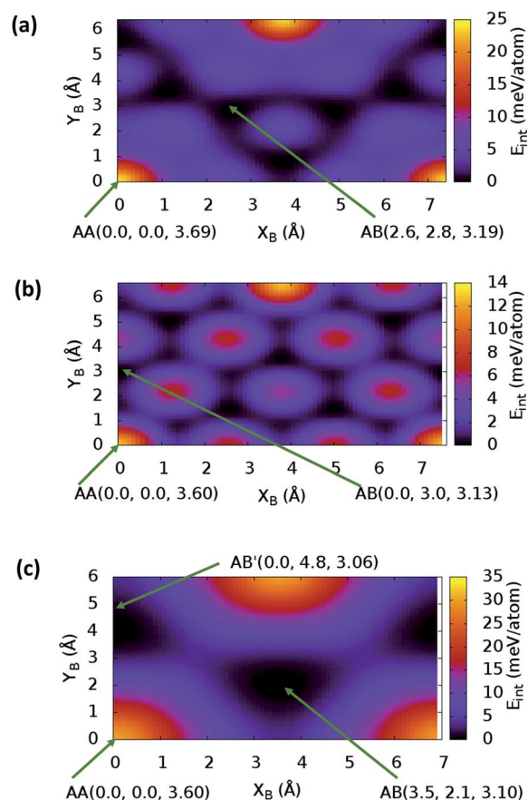
Fig. 2 Stacking energy profile for (a) bulk \text{C}_{12}\text{H}_6\text{-h2D} , (b) bulk \text{B}_6\text{N}_6\text{H}_6\text{-h2D} , and (c) bulk \text{C}_6\text{N}_6\text{-h2D} . ( X_B , Y_B ) is the shift in the top layer relative to the bottom layer. ( X_B = 0 , Y_B = 0 ) corresponds to the AA stacking. AB' denotes the most stable stacking in \text{C}_6\text{N}_6\text{-h2D} , which corresponds to neither AA nor AB. E_{\text{int}} values presented are relative to the most stable stacking configuration.
