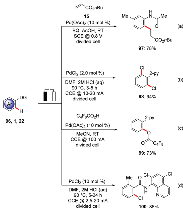
Scheme 34 Palladaelectro-catalyzed C–H activation.
