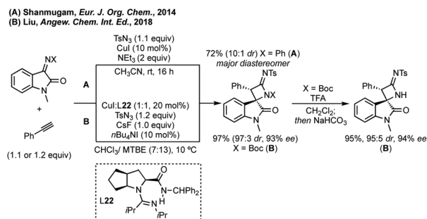
Scheme 20 Cu-Catalysed one-pot, three component synthesis of spiroazetidininone oxindoles from isatin derived ketimines.
