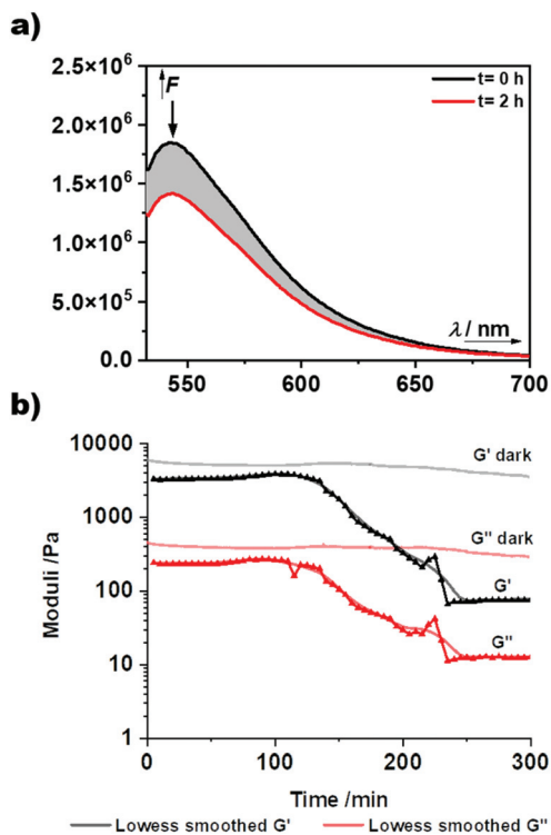
Fig. 4 Kinetic studies of the photodegradation of the BODIPY-diol containing hydrogel. (a) Decrease of the fluorescence intensity upon irradiation of the BODIPY-hydrogel at 510 \text{ nm} for 2 \text{ h} . (b) Photorheology measurements of the BODIPY-hydrogel and the stability of the gel in the dark. Light on after 2 \text{ min} .
