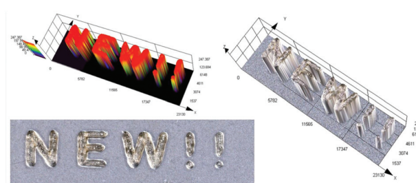
Fig. 14 3D hydrogel inscription made by the free-radical photopolymerization of a HEA/water (1/1 wt%) mixture in the presence of a two-component photoinitiating system based on CA-CDs (0.2 wt%) and IOD (2 wt%).
