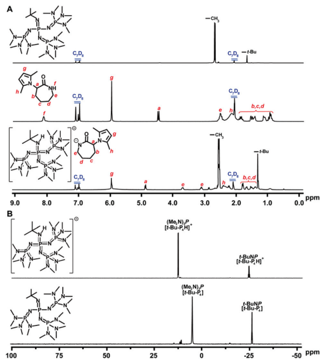
Fig. 4 (A) ^1\text{H} NMR spectra (toluene- d_8 , 25 ^\circ\text{C} ) of the reaction between t\text{-Bu}_4\text{P} and M5 (1 : 1). (B) ^{31}\text{P} NMR spectra (toluene- d_8 , 25 ^\circ\text{C} ) of the reaction between t\text{-Bu}_4\text{P} and M5 (1 : 1). Reproduced from ref. 26 with permission from the American Chemical Society, copyright 2017.
