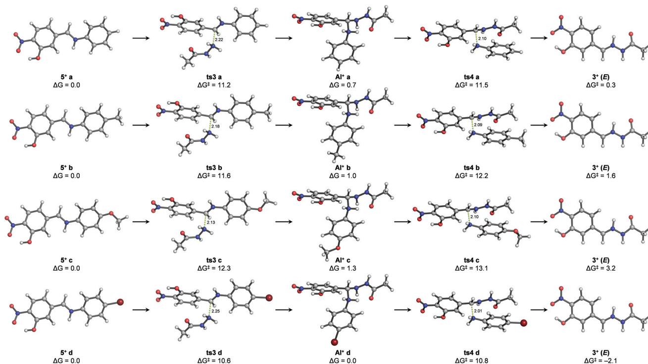
Fig. 5 Lowest-energy structures calculated with SMD(CH 3 CN)/M06-2X/6-311++G(2d,p)//PCM(CH 3 CN)/M06-2X/6-31+G(d,p) for the nucleophilic addition of acylhydrazide to iminium derivatives 5 * a–d ( ts3 a–d ) and subsequent aminal intermediates ( Al + a–d ) and subsequent water elimination ( ts4 a–d ) to yield hydrazone 3 + (only the E isomer is shown). Relative free energies ( \Delta G ) from the separated reactants are given in kcal·mol -1 and distances are given in Angstrom.
