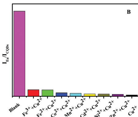
Fig. 5 (A) The emission spectra and the relative intensities of I_{613}/I_{450} for Eu-DPA-CQDs dispersed in different metal ion ( 10^{-3} \text{ mol L}^{-1} ) aqueous solutions. (B) I_{Eu}/I_{CQDs} of 500 \text{ }\mu\text{M Cu}^{2+} ions and various co-existing metal ions.
