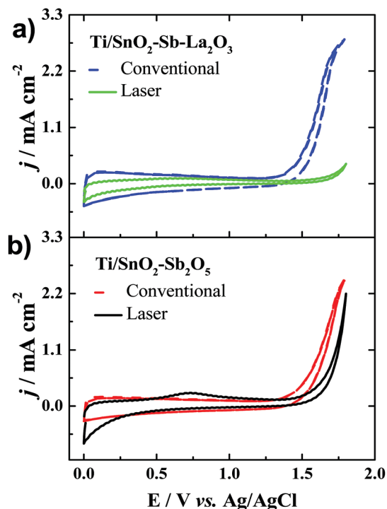
Fig. 5 Cyclic voltammograms recorded at 50 \text{ mV s}^{-1} for the anodes of (a) \text{Ti/SnO}_2\text{-Sb-La}_2\text{O}_3 and (b) \text{Ti/SnO}_2\text{-Sb}_2\text{O}_5 . Electrolyte: 0.5 \text{ mol L}^{-1} \text{ H}_2\text{SO}_4 .
