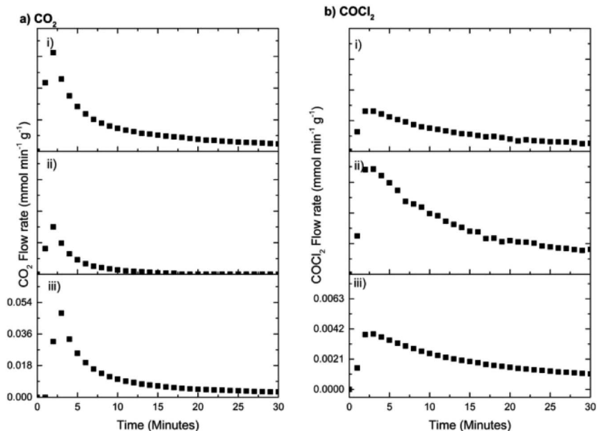
Fig. 16 (a) \text{CO}_2 and (b) \text{COCl}_2 formation rates on continuous dosing of CO at 653 K as a function of time-on-stream after three sets of chlorine pre-treatments with a fixed aliquot of 12.8 mmol \text{Cl}_2 per g_{(\text{cat})} . Run (i) corresponds to a single exposure of 12.8 mmol \text{Cl}_2 per g_{(\text{cat})} prior to monitoring the reaction with CO. Run (ii) corresponds to an additional exposure of 12.8 mmol \text{Cl}_2 per g_{(\text{cat})} again prior to reaction with CO. Upon completion of run (ii) the catalyst experienced a further dichlorine pre-treatment (12.8 mmol \text{Cl}_2 per g_{(\text{cat})} ) prior to the reactor being purged with nitrogen for 30 min. Heating was then switched off, the reactor was isolated, and the catalyst was cooled to 293 K and left overnight in an inert atmosphere. After 12 h, the reaction with CO was repeated as normal at 653 K. Flow conditions: CO 5 \text{ cm}^3 \text{ min}^{-1} , \text{N}_2 (carrier gas) 54 \text{ cm}^3 \text{ min}^{-1} , and \text{N}_2 (diluent post-reactor) 100 \text{ cm}^3 \text{ min}^{-1} .
