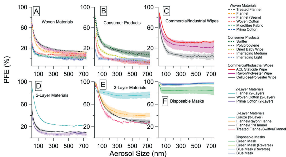
Fig. 3 PFE as a function of aerosol size for all tested materials and multi-layer combinations, grouped according to material class: (A) woven materials; (B) consumer products; (C) the commercial/industrial wipes; (D) 2-layer materials; (E) 3-layer materials; and (F) disposable masks. Variability shown is one standard deviation of the mean for the three tests.
