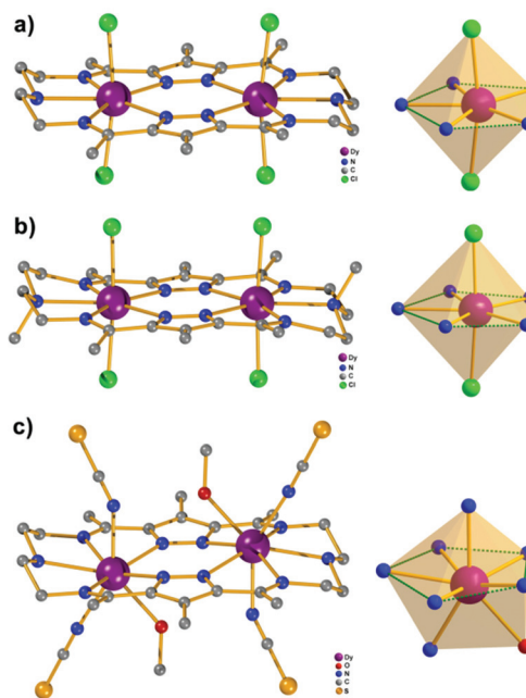
Fig. 2 Structure views of complexes \text{Dy}_2\text{-Cl} (a), \text{Dy}_2^+\text{-Cl} (b), and \text{Dy}_2\text{-NCS} (c). The orange spheres represent the coordination polyhedron of the relevant \text{Dy}^{\text{III}} ion in the complexes. Hydrogen atoms are omitted for clarity.
