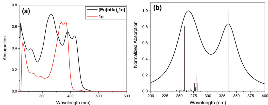
Fig. 2 (a) Optical absorption spectra of 1c and [\text{Eu}(\text{btfa})_3]1\text{c} at RT. (b) Theoretical electronic spectrum calculated at the CAM-B3LYP level of theory using the B3LYP geometry for [\text{Eu}(\text{btfa})_3]1\text{c} .
