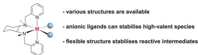
Chart 7 Summary of features of water oxidation catalysts with alkylamine-pyridine ligands.
