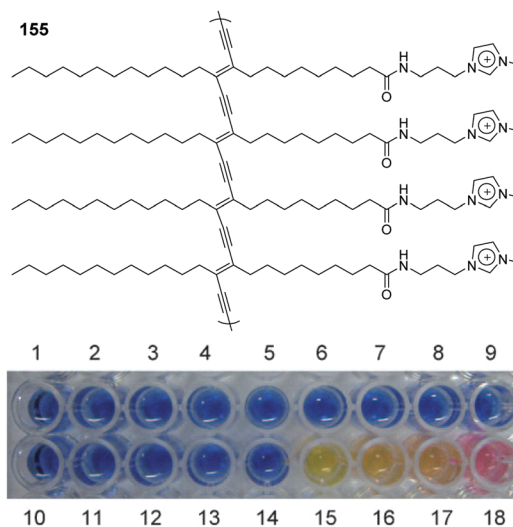
Fig. 14 Structure of polymerized 155 (100 \mu\text{m} ) and colorimetric responses of polymerized 155 (100 \mu\text{m} ) in the presence of various analytes (500 \mu\text{m} ) in HEPES buffer (20 mM, pH 7.4): 1 blank, 2 \text{F}^- , 3 \text{Cl}^- , 4 \text{Br}^- , 5 \text{I}^- , 6 \text{SO}_4^{2-} , 7 \text{CO}_3^{2-} , 8 \text{ClO}_4^- , 9 \text{CH}_3\text{COO}^- , 10 \text{NO}_3^- , 11 \text{HPO}_4^{2-} , 12 \text{SCN}^- , 13 CTAC, 14 Triton X-100, 15 SDS, 16 SDC, 17 SDP, 18 SDBS.
