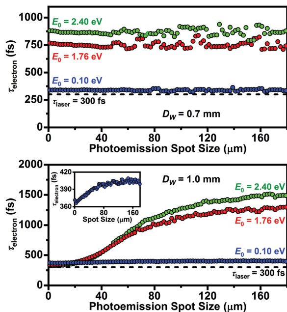
Fig. 2 Single-electron-packet duration ( \tau_{\text{electron}} ; fwhm) as a function of \text{LaB}_6 photoemission spot size for D_W = 0.7 mm (top) and D_W = 1.0 mm (bottom). Note that three discrete initial photoelectron kinetic energies ( E_0 = 0.10, 1.76, and 2.40 eV) were compared ( i.e. , here, the full distributions shown in Fig. 1d were not yet used in order to first focus on the effect of photoemission spot size and D_W ). The horizontal black dashed line in each panel ( \tau_{\text{laser}} ) represents the selected probe laser-pulse duration of 300 fs (fwhm) typical of the current system at Minnesota. The inset (bottom panel) is the 0.10 eV plot for D_W = 1.0 mm with the y -axis rescaled to visualize the subtle response of \tau_{\text{electron}} .
