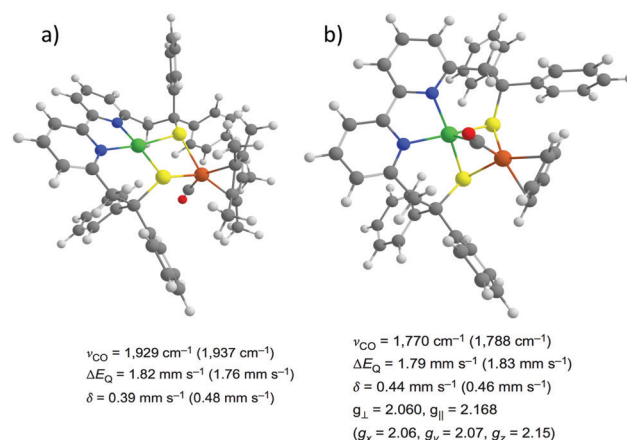
Fig. 13 Structures of the biomimetic models for the Ni-S1a (a) and Ni-L (b) states of the [NiFe] hydrogenase identified by combining spectroscopic measurements and DFT computations. Adapted with permission from ref. 40. Copyright 2016 Nature Publishing Group.
