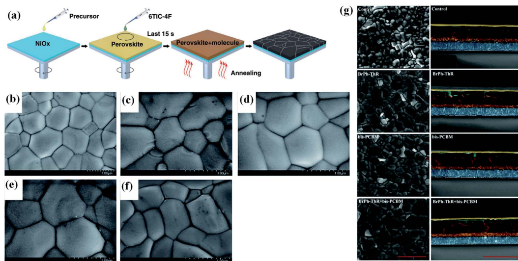
Fig. 8 (a) Schematic diagram of the deposition processes of the prepared CsPbBr_{x-1}Br_{1-x} perovskite film. Reproduced by the permission of ref. 82, Copyright 2020, Springer Nature. Top-view scanning electron microscope images of (b) CsPbBr_3 , (c) CsPb_{0.97}Mg_{0.03}Br_3 , (d) CsPb_{0.97}Ca_{0.03}Br_3 , (e) CsPb_{0.97}Sr_{0.03}Br_3 and (f) CsPb_{0.96}Ba_{0.04}Br_3 films. Reproduced by permission ref. 84, Copyright 2019 Royal Society of Chemistry. (g) SEM images. Top (left, the scale is 1 \mu m ) SEM of corresponding perovskite films and cross-sectional (right, the scale is 2 \mu m ) SEM of corresponding perovskite devices. (1) Control; (2) BrPh-ThR; (3) bis-PCBM; and (4) BrPh-ThR + bis-PCBM. Reproduced by permission ref. 85, Copyright 2018 Royal Society of Chemistry.
