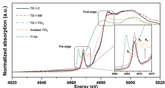
Fig. 4 Ti K-edge XANES spectra of different TS-1 samples, anatase \text{TiO}_2 , and Ti foil reference.
