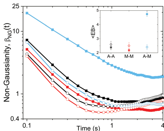
Fig. 4 Non-Gaussianity parameter, \beta_{\text{NG}}(t) and ergodicity-breaking term, EB, show that DNA transport dynamics are both non-Gaussian and non-ergodic. \beta_{\text{NG}} versus time for both linear (closed squares) and ring (open circles) DNA diffusing in networks comprised of actin-actin (A-A, black), microtubule-microtubule (M-M, red), and actin-microtubule (A-M, light blue) crosslinking. Inset: Time-average of the corresponding ergodicity-breaking term EB. Note that both \beta_{\text{NG}} and EB are zero for a particle undergoing normal Brownian diffusion. See text for definitions of \beta_{\text{NG}} and EB.
