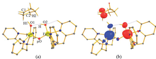
Fig. 5 (a and b) The optimised structure of I^{-2}Int_{hh-hs} and its corresponding spin density plot. Some important structural parameters computed for the spin states and spin density values are given below for species I-Int . For spin state ^2Int_{hh-hs} , Fe^{III}-O1 = 1.854 , Fe^{III}-O2 = 1.835 , Fe^{III}-\mu O = 1.806 , Fe^{III}-\mu O1 = 1.825 , O1-H1 = 0.981 , H1-C1 = 2.012 , \angle Fe^{III}-O1-H1 = 129^\circ , and \angle O1-H1-C1 = 167^\circ and spin density Fe^{III} = -3.97 , Fe^{III} = 3.96 , O1 = -0.25 , O2 = 0.38 , \mu O = -0.07 , and C1 = 0.93 . All the distances are given in Å and angles in ^\circ . All hydrogen atoms (except O2-H , C1-H1 , and C2-H2 ) are omitted for clarity.
