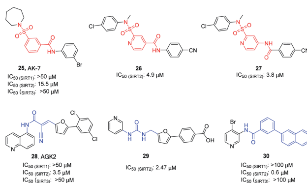
Fig. 5 Chemical structures of 3-benzenesulfonylaminobenzamide-based SIRT2 inhibitors and their inhibitory activity data on SIRT2 by Fluor-de-Lys fluorescent assays. 45,46
