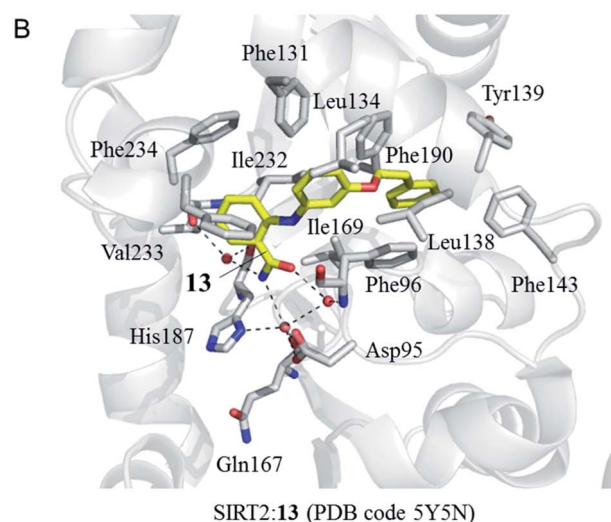
Fig. 3 (A) Chemical structures of nicotinamide-based SIRT2 inhibitors and their inhibitory activity data on SIRT2 determined by Fluor de Lys assays. 34 (B) Crystallographic analyses revealed the binding features of 13 with SIRT2.
