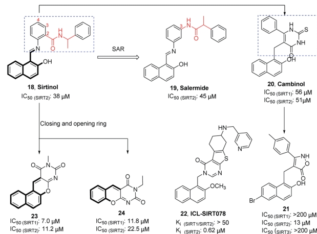
Fig. 4 Chemical structures of hydroxynaphthaldehyde-based SIRT2 inhibitors and their inhibitory activity data on SIRT2 by fluorescence-based or SIRT-Glo assays. 38–40
