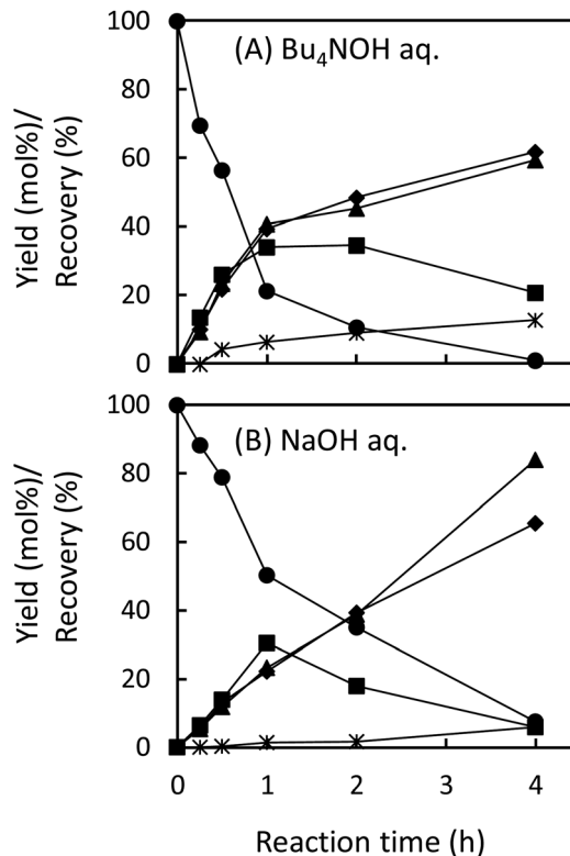
Fig. 5 Changes with time in recovery of LM2 (●), yields of guaiacol (◆), vanillin (▲), vanillic acid (*), and enol ethers EEs a (■) during degradation of LM2 (5.0 mg) at 120 °C under air in 1.25 \text{ mol L}^{-1} Bu 4 NOH aq. (1.0 mL) (A) and in 1.25 \text{ mol L}^{-1} NaOH aq. (1.0 mL) (B). a The yields of EEs are shown as the sum of the cis - and trans -isomers.
