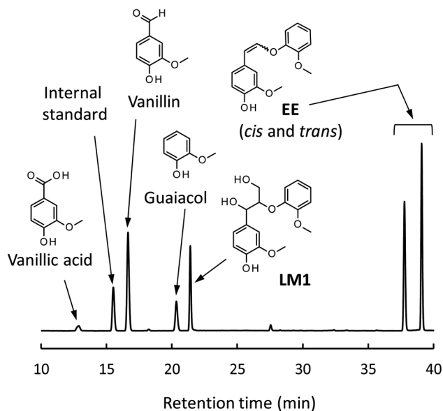
Fig. 4 HPLC chromatogram of the reaction mixture obtained after the degradation of LM2 (5 mg) in 1.25 \text{ mol L}^{-1} Bu 4 NOH aq. (1.0 mL) under air for 1 h.
