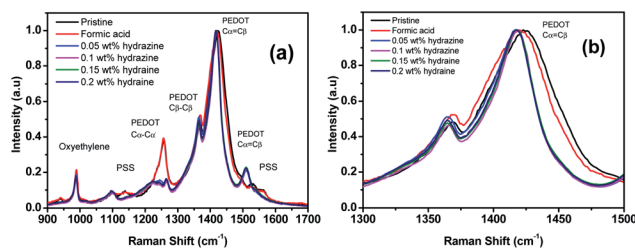
Fig. 7 (a) Raman spectra of the PEDOT:PSS films before and after treatment with formic acid and formic acid-hydrazine. (b) The zoomed spectra for the wavenumbers ranging from 1300 to 1500 \text{cm}^{-1} .
