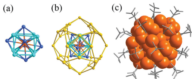
Fig. 16 (a) The \text{Ag}@\text{Ag}_{14} core; (b) the structure of the \text{Ag}@\text{Ag}_{14}@\text{Ag}_{36} shell; and (c) overall structure of \text{Ag}_{51}({}^t\text{BuC}\equiv\text{C})_{32} . Adapted with permission from ref. 36. Copyright 2018, Royal Society of Chemistry.
