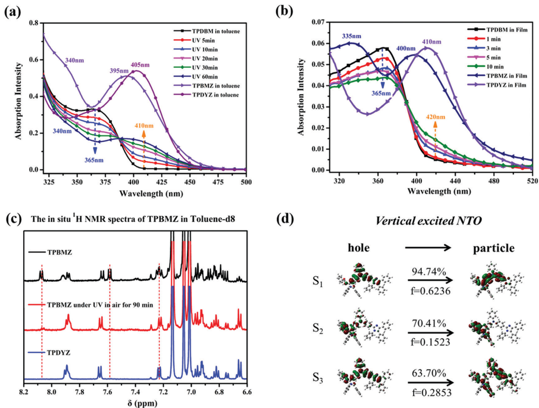
Fig. 6 In situ UV spectra of TPBDM (a) in toluene solution and (b) as a film. (c) In situ 1 H NMR spectra of TPBMZ. (d) The natural transition orbital (NTO) distributions of TPBMZ relating to S 0 → S 1 , S 0 → S 2 and S 0 → S 3 excitations at the TD-ob97X/6-31G(d,p) level using S 0 state geometry.
