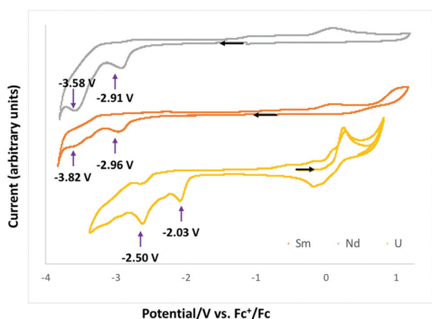
Fig. 4 Cyclic voltammogram of complexes 1-Nd (grey), 1-Sm (orange) and 1-U (yellow) from ref. 10c in ~0.1 M [Bu_4N][PF_6] THF solution at a 100\text{ mV s}^{-1} scan rate.
