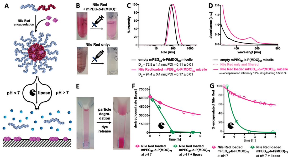
Fig. 6 Nile Red formulated into m\text{PEG}_{48}\text{-}b\text{-P}(\text{MDO})_{50} micelles. (A) Schematic representation of Nile Red loading and release. Under acidic and basic conditions, micellar degradation is highly accelerated. Upon degradation, Nile Red is expected to be released and precipitate. (B) Nile Red formulated with and without the polymer. Pictures are shown before and after filtration ( 450\ \mu\text{m} ). Whereas Nile Red formulated with the polymer is stabilized in solution, Nile Red was solely removed by filtration leading to a clear colourless solution. (C) DLS measurement and (D) UV/Vis absorbance spectra of micelles formulated with and without Nile Red. (E) Photograph of Nile Red loaded particles before and after degradation. (F) Lipase-mediated enzymatic degradation of Nile Red loaded m\text{PEG}_{48}\text{-}b\text{-P}(\text{MDO})_{71} micelles followed by the light scattering count rate. (G) Lipase-mediated Nile Red release from m\text{PEG}_{48}\text{-}b\text{-P}(\text{MDO})_{71} micelles followed by UV-vis absorbance at 549\ \text{nm} .
