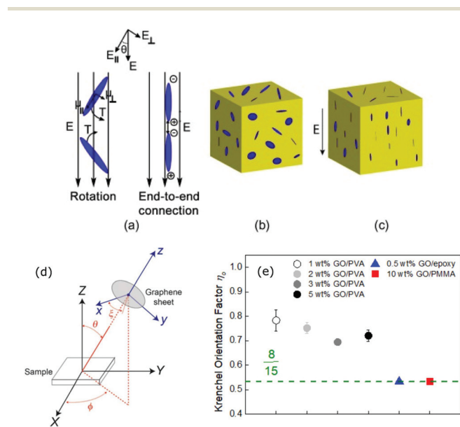
Fig. 5 Two different alignment mechanisms of the GNPs by an AC electric field through: (a) rotation (left) and end-to-end connection (right) of polarized GNPs, (b) initial random orientation of GNPs within an epoxy resin, (c) oriented GNPs along the electric field direction within the resin 71 (Copyright 2015, with permission from Elsevier), (d) the relationship between the local coordinate system of a graphene sheet ( x, y, z ) and the nanocomposite ( X, Y, Z ) defined by the three Euler angles ( \theta, \phi, \xi ). 77 (e) Krenchel orientation factor of the composites studied in ref. 77 (the dashed line represents the Krenchel factor of 8/15 for the materials reinforced with randomly distributed GNPs (Copyright 2016, with permission from Elsevier).
