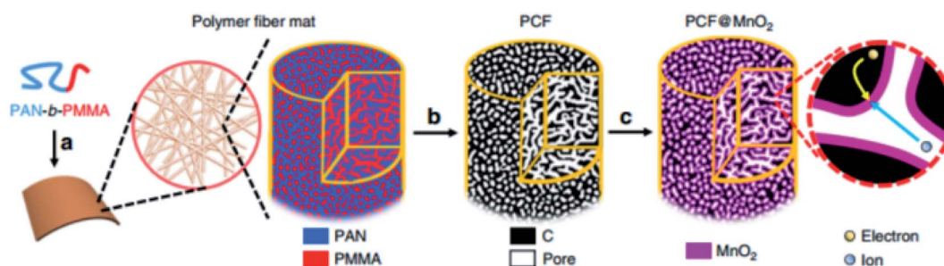
Fig. 2 Schematic illustration of the synthesis of PCF and PCF@MnO_2 . (a) PAN-b-PMMA block copolymer is spun into a polymer fiber mat. (Magnified view) PAN (blue) and PMMA (red) in the block copolymer fiber microphase separate into a bicontinuous network structure. Via thermal oxidation, PAN is crosslinked to ensure a high yield of conductive carbon network. (b) Upon pyrolysis, the polymer fibers are converted to porous carbon fibers (PCFs, black) with continuous and uniform mesopores (white channels), which afford high loadings of transition metal oxides. (c) The PCFs are loaded with MnO_2 (magenta) to become PCF@MnO_2 through a solution-based redox deposition reaction. (Magnified view) The continuous carbon fiber matrix and the partially filled mesoporous channels provide effective expressways for electron conduction and ion diffusion, respectively. 65
