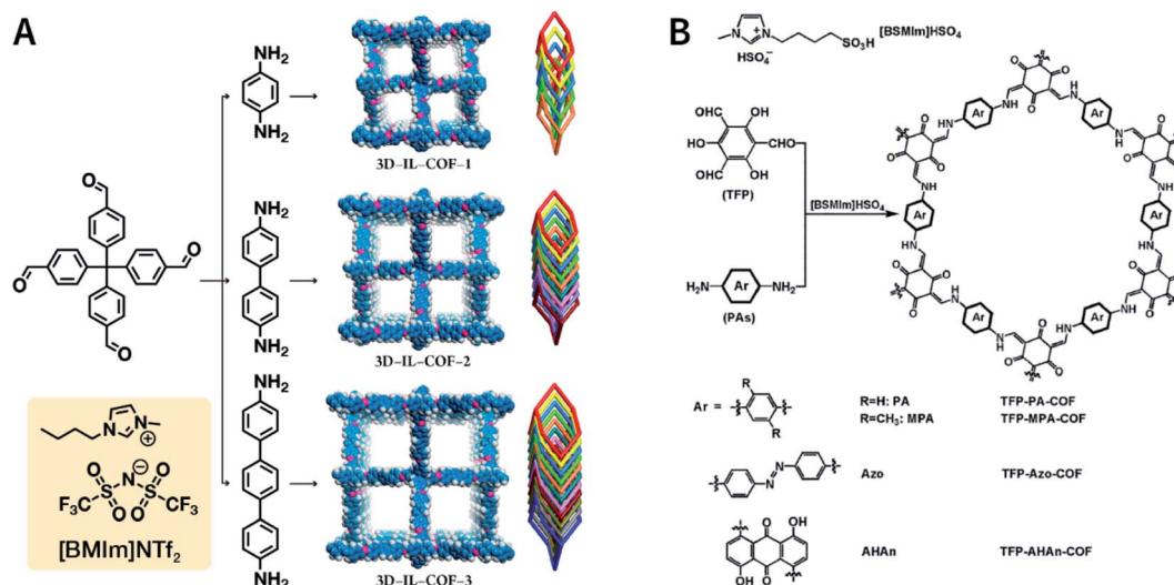
Fig. 12 Ionothermal synthesis of COFs. (A) Synthesis of 3D COFs in [BMIIm]NTf 2 IL. Adapted with permission. 115 Copyright 2018, American Chemical Society. (B) Synthesis of \beta -ketoenamine-linked COFs in [BSMIm]HSO 4 IL. Adapted with permission. 116 Copyright 2019, Elsevier B.V.
