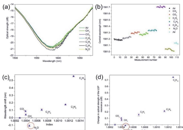
Fig. 6 Typical experimental results of a UV processed Ge/SiO_2/Pt LSP fibre device coated with SWNTs as a function of surrounding refractive index and nitrous oxide (a) the transmission spectra as function of surrounding gas. (b) The individual measurements of the central wavelength of the LSP resonance for each alkane gas and nitrous oxide (c) and (d) the wavelength and optical strength sensitivity as a function of the different gas's refractive index respectively.
