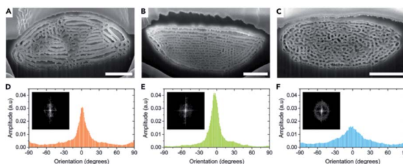
Fig. 4 The Sulawesiella rafaelsae longhorn beetle displays orange (A and D), green (B and E) and turquoise (C and F) coloured areas due to perforated multilayer structures embedded in the scales covering the beetle elytra. Based on SEM images of the scale cross-sections (A–C), variable distributions in the layer orientations (D–F) were measured and 2D-FFT analyses were performed (insets in D–F). The different extents of disorder in these scales give rise to various iridescence and scattering properties. Scale bars: 2 \mu\text{m} (A–C). Reproduced from ref. 52, License CC-BY-NC-ND.
